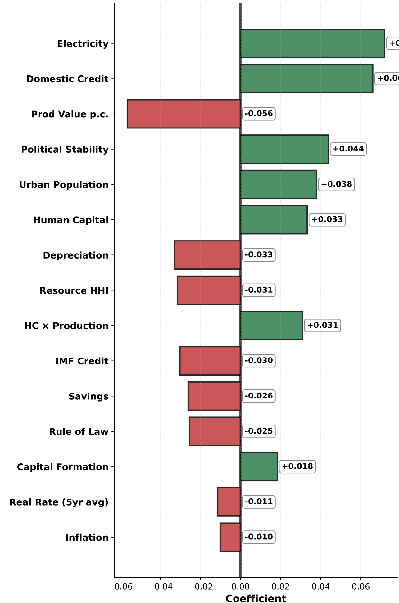
Ridge Train R 2 =0.783 Test R 2 =0.849 | 23 features
