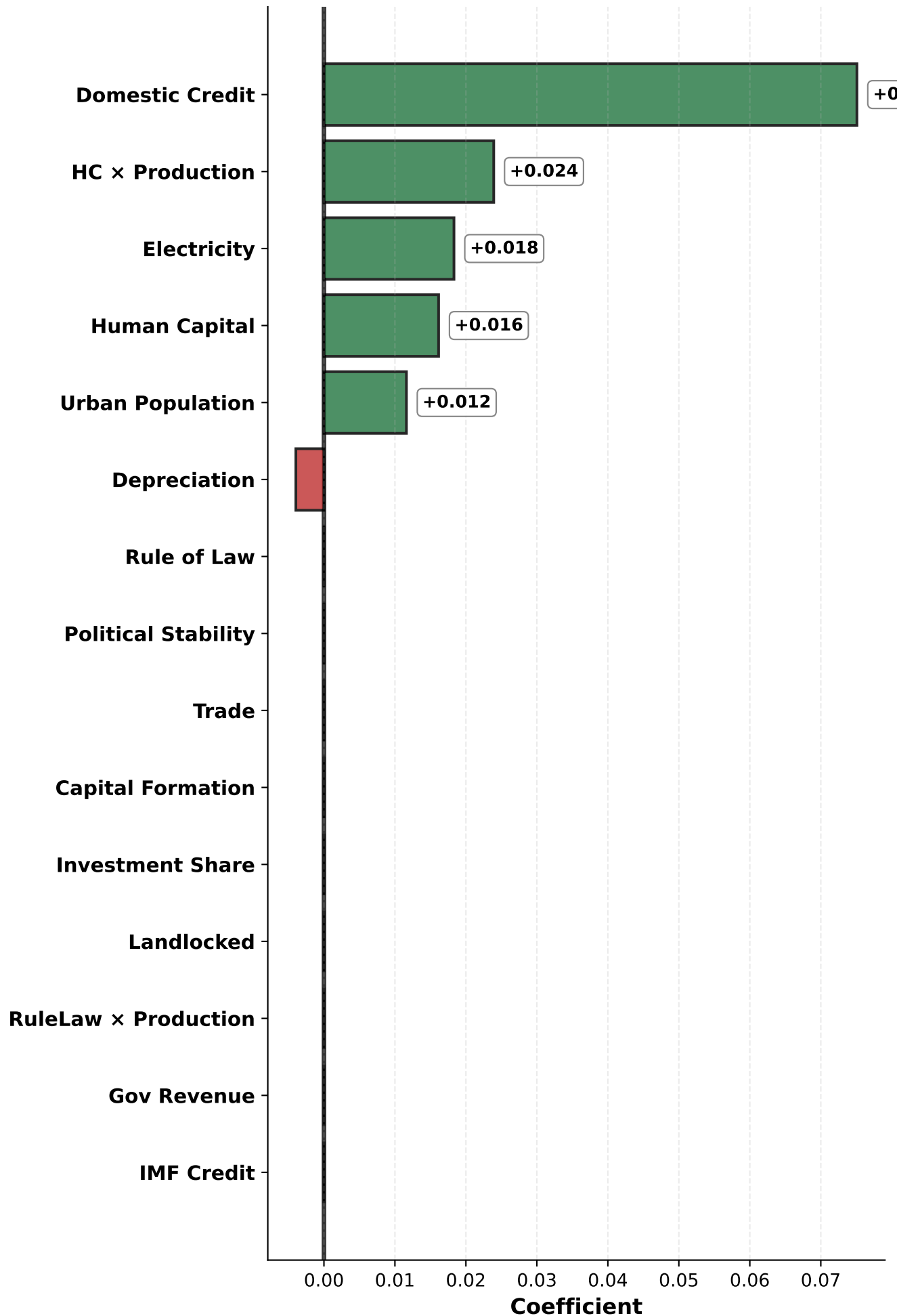
Elastic Net Train R 2 =0.771 Test R 2 =0.855 | 7 features
